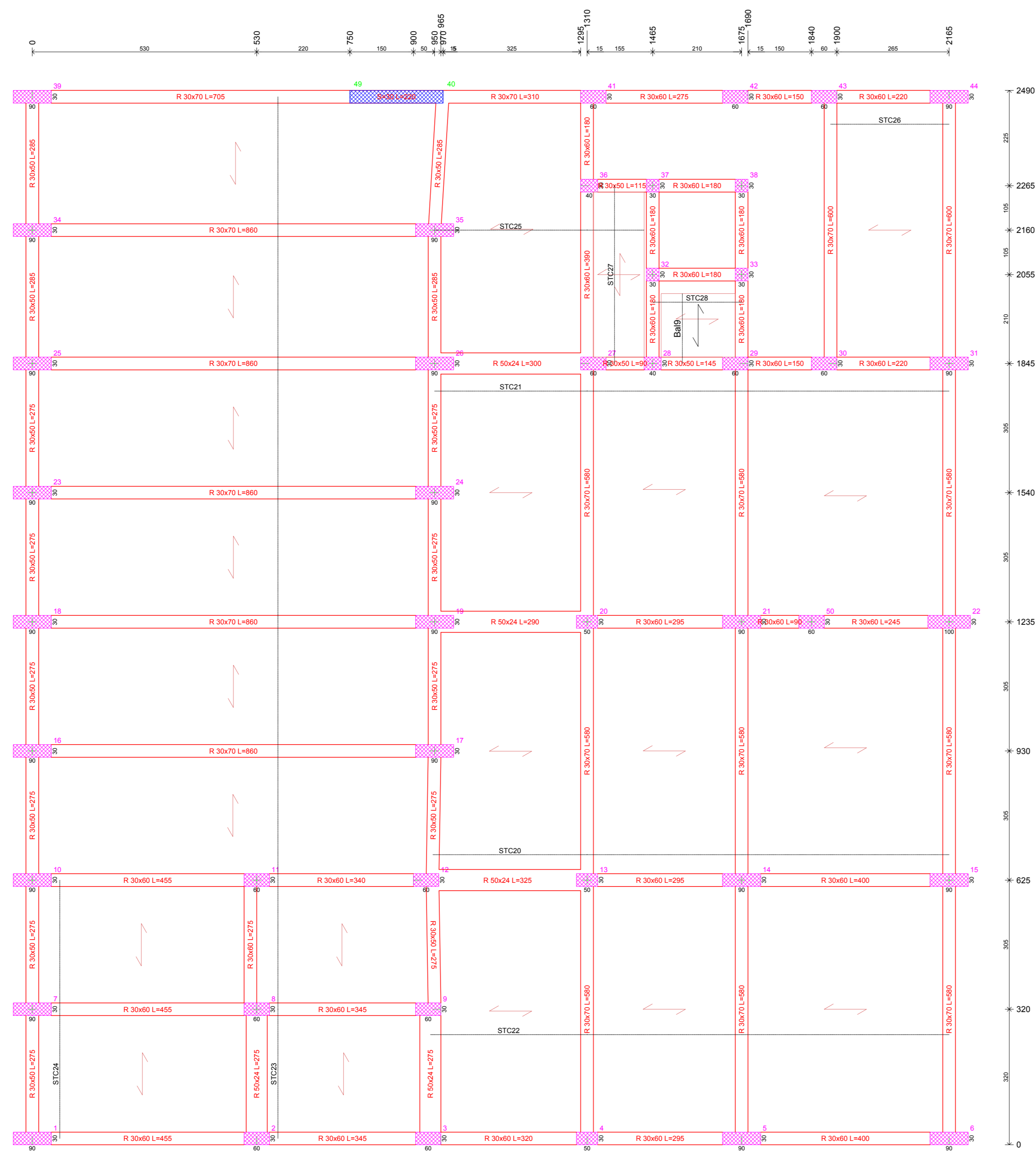
Carpenteria Piano 3 (Scala 1:50)
