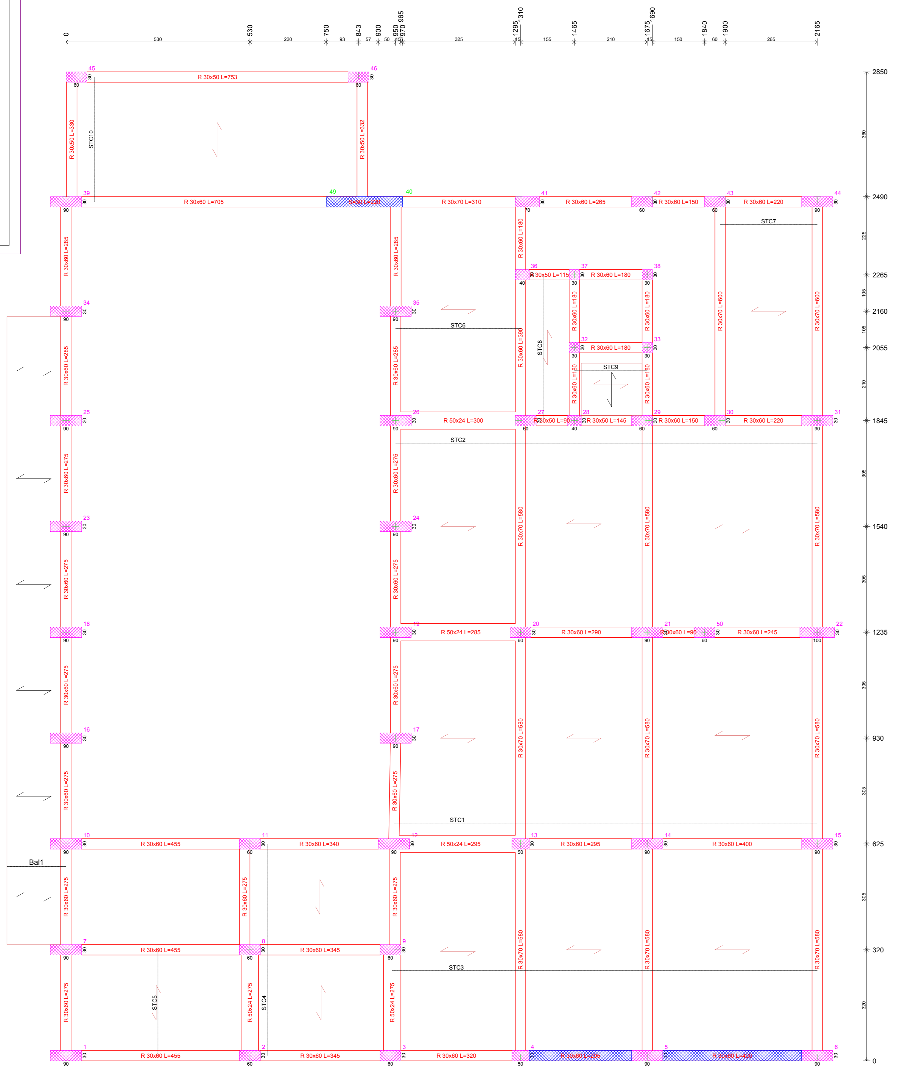
Carpenteria Piano 1 (Scala 1:50)
